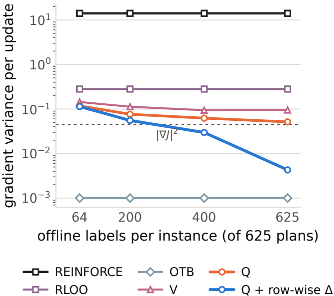
What the reward model costs
