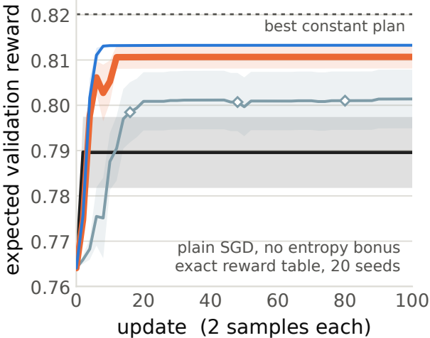
learning curve, lr 0.5
