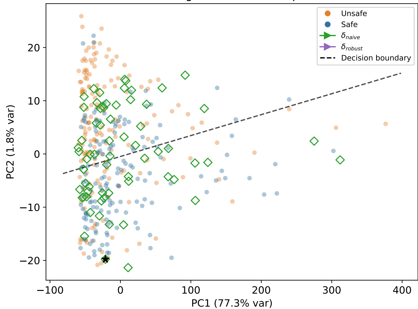
Steering Vectors in PCA Space
