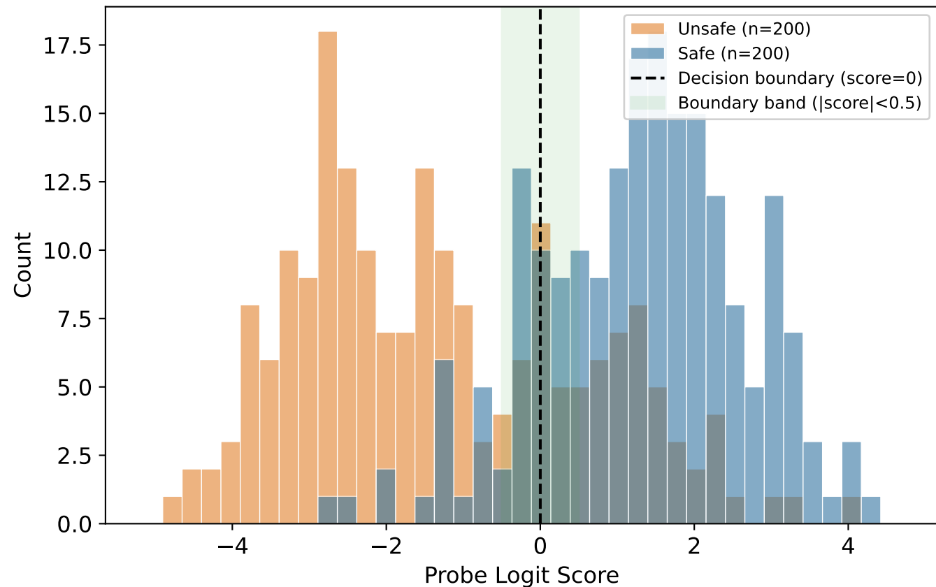
IT-Model Probe Score Distribution
