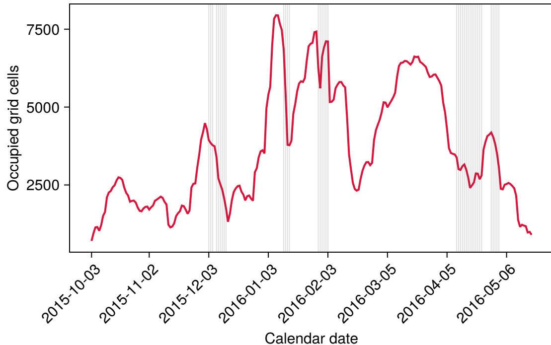
Original event size
