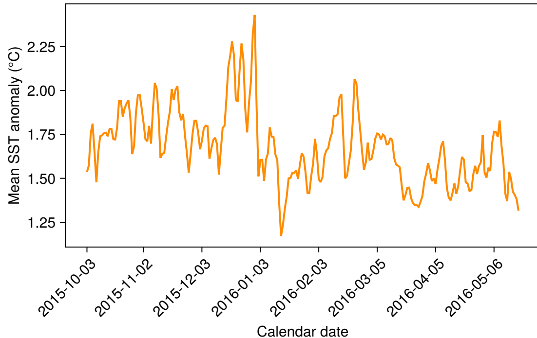
SST anomaly within the tracked event
