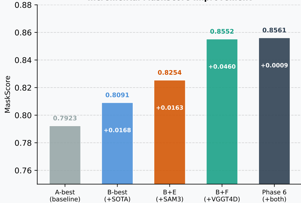
Incremental MaskScore Improvement
