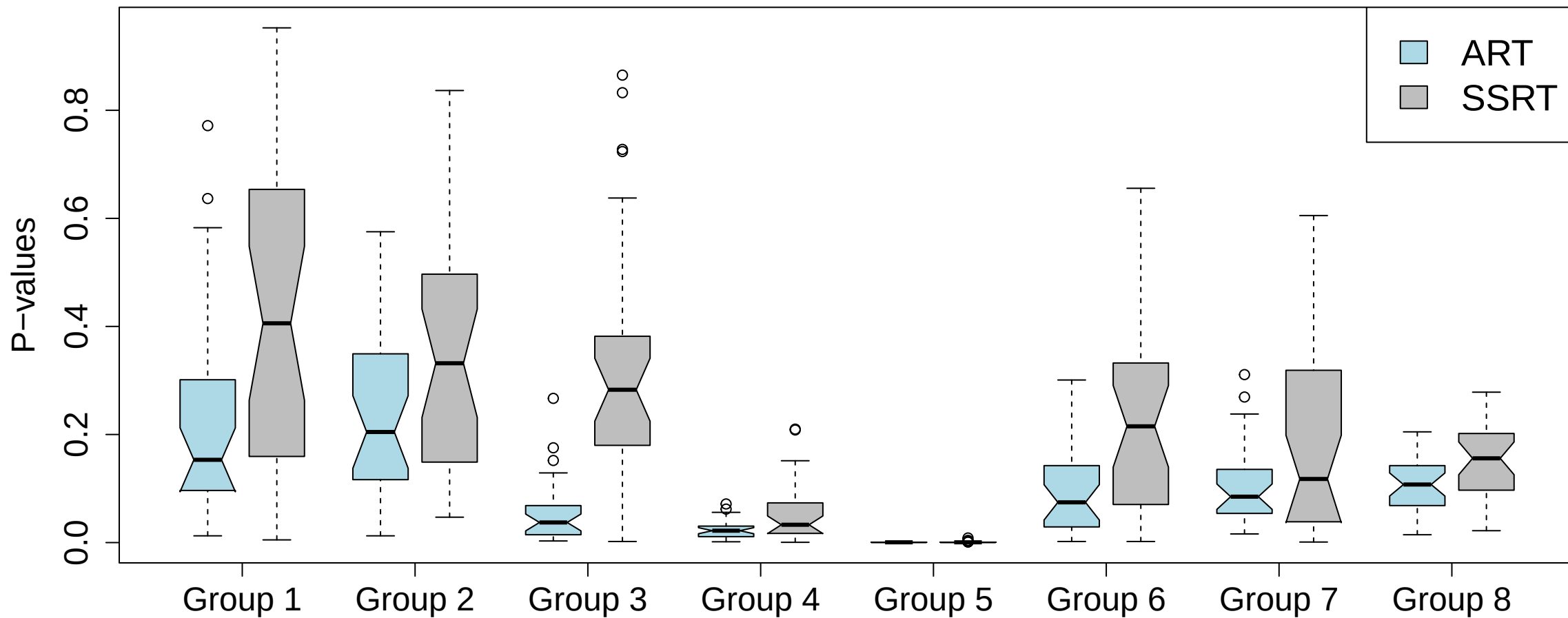
Comparison of ART and SSRT (Inference fold: 10%)
