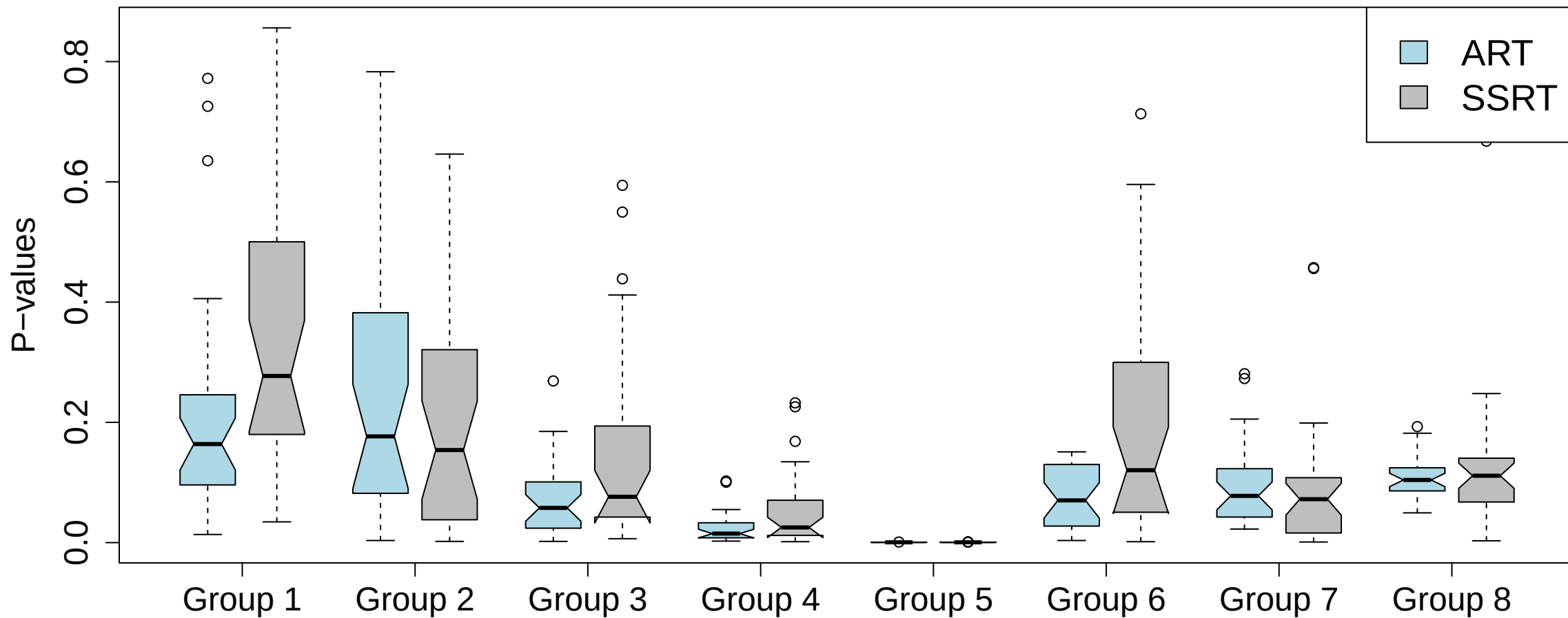
Comparison of ART and SSRT (Inference fold: 20%)
