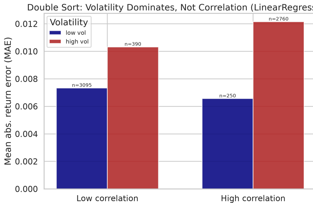
Figure 6. Mean absolute error by correlation and volatility cell.
