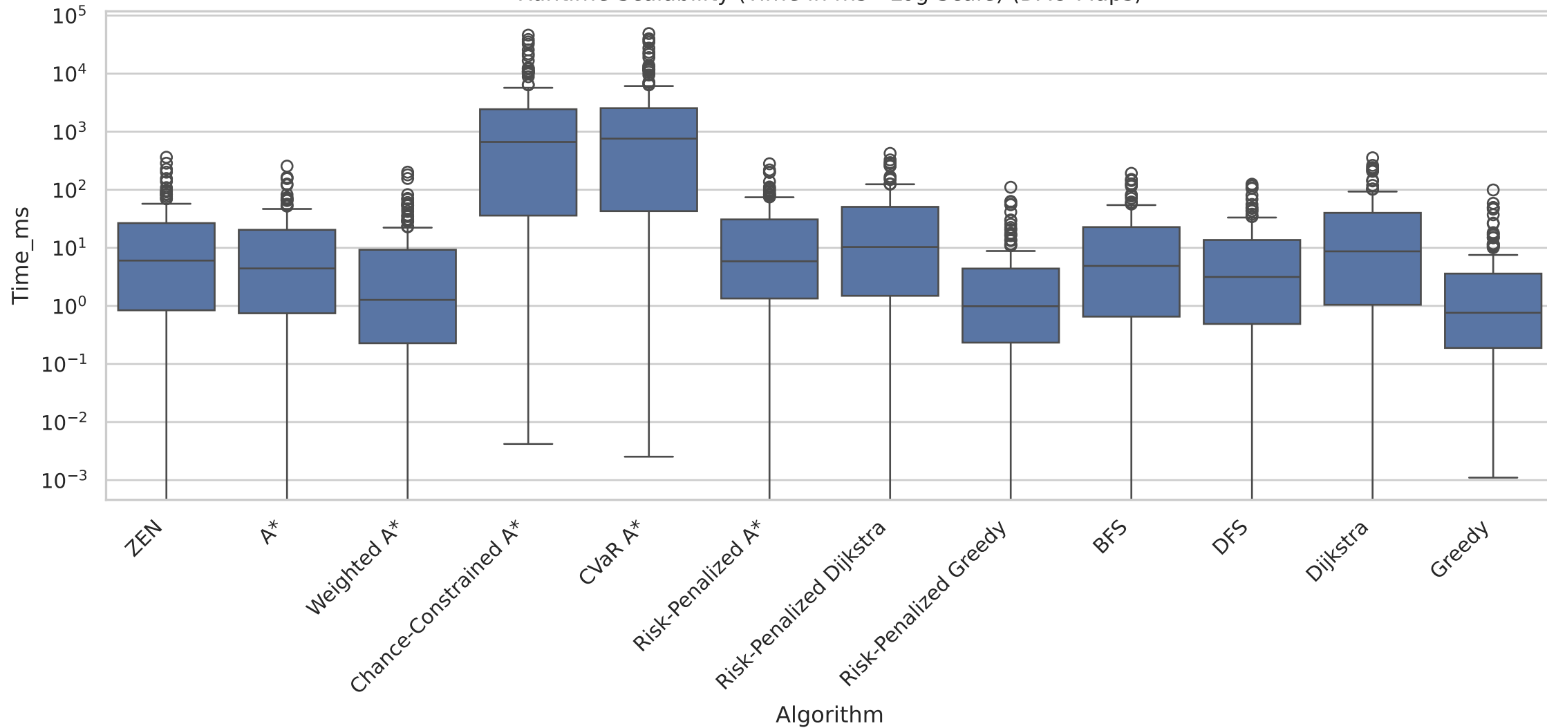
Runtime Scalability (Time in ms - Log Scale) (DAO Maps)
