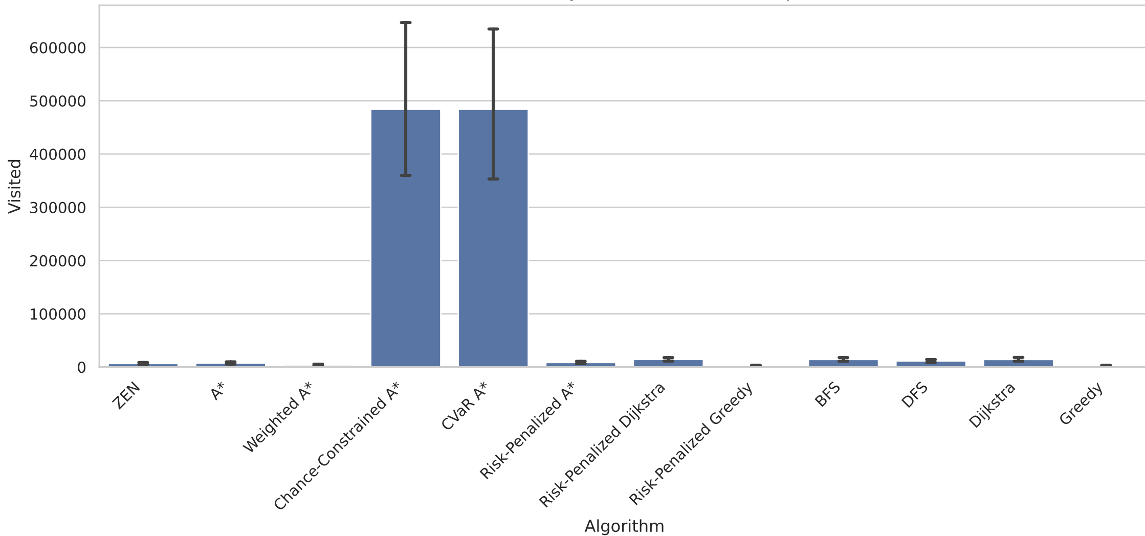
Search Efficiency (Nodes Visited) (DAO Maps)
