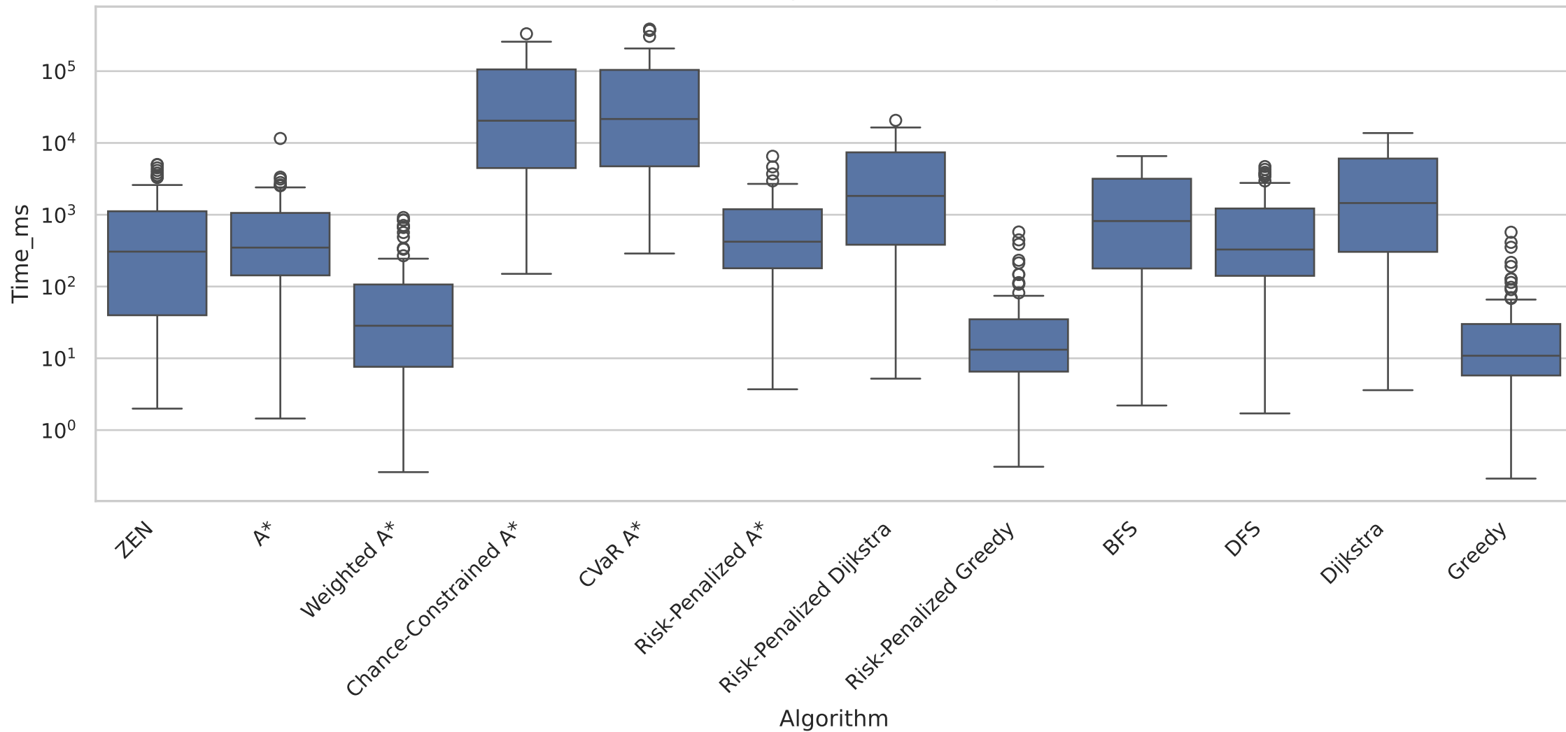
Runtime Scalability (Time in ms - Log Scale)
