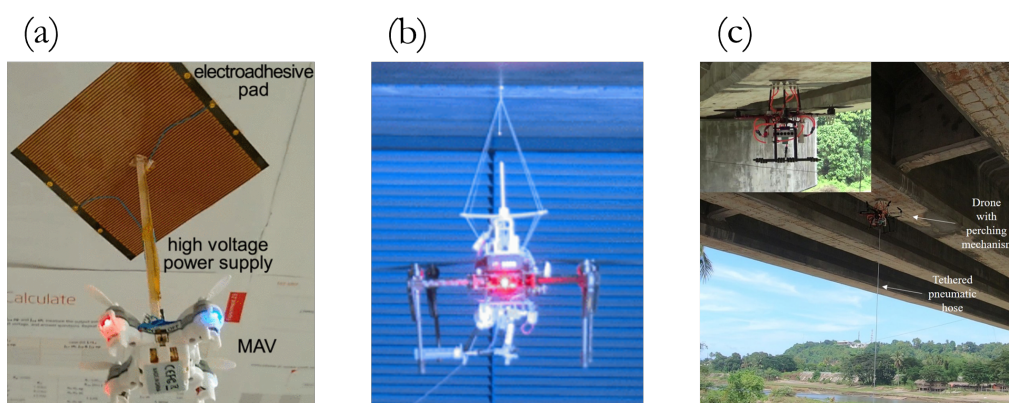
图 1.3 部分基于黏附的栖息无人机设计, (a) [21] , (b) [21] , (c) [21]
