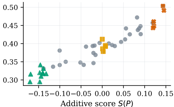
k=3: uniform \rho=0.921
