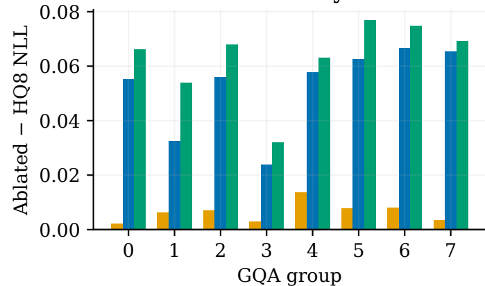
Discovery
