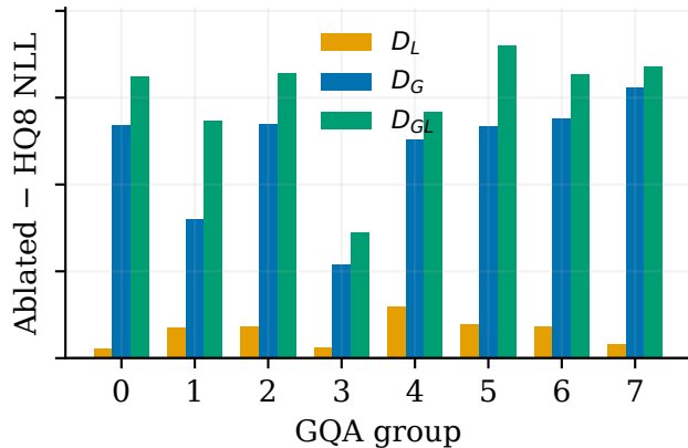
Confirmation
