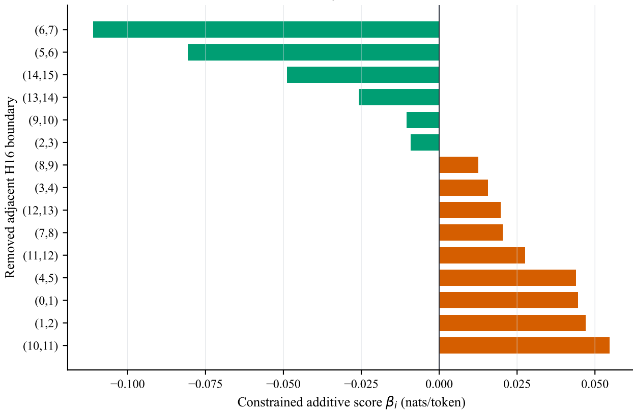
Relative boundary-removal scores at k=4
