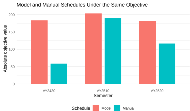
Figure 4: Model and manual schedules compared by absolute objective value across three semesters. Both schedules are scored using the same policy weights. Taller bars represent more negative, and hence lower, objective values; under this policy, the optimized model schedule has a lower weighted objective than the manual schedule in all three semesters.
