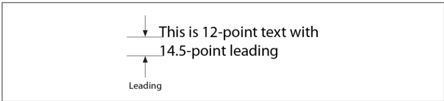
Figure 59 — Leading
