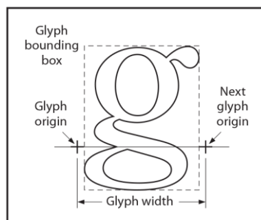
Figure 54 — Glyph metrics
