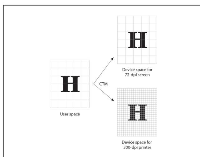
Figure 11 — User space
