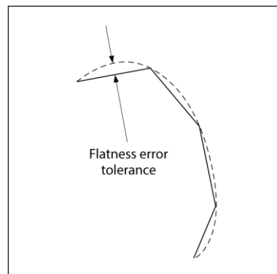
Figure 69 — Flatness tolerance
