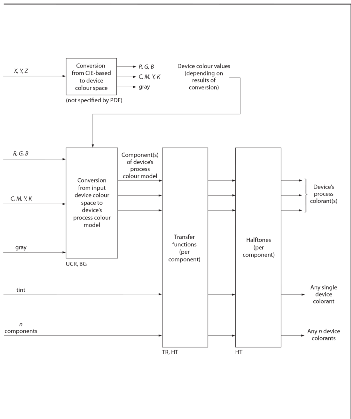
Figure 21 — Colour rendering
