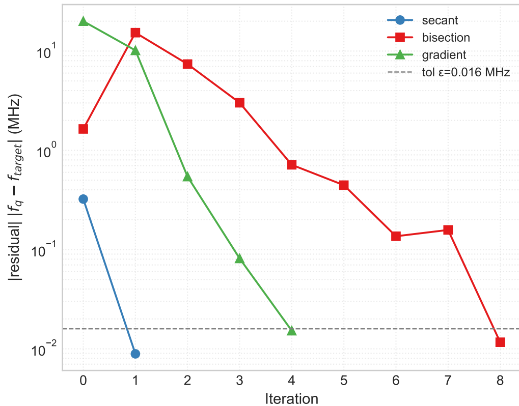
Closed-loop convergence (target -20 MHz)
