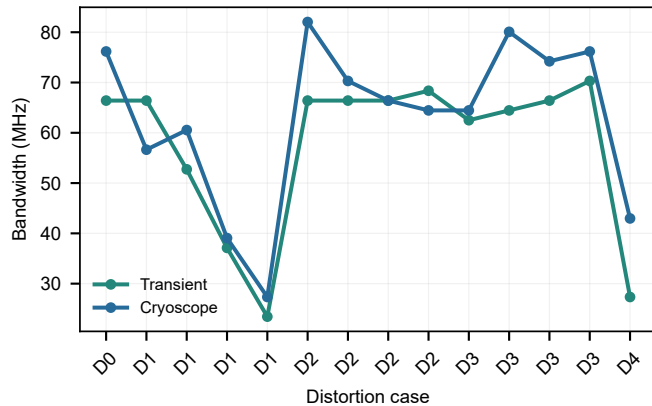
(d) Qualified bandwidth across distortion cases
