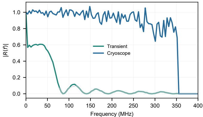
(d) Qualified bandwidth across distortion cases
