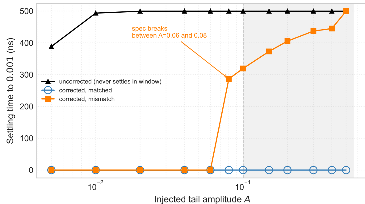
(c) Settling spec: correction holds to A \approx 0.06 , then degrades toward the uncorrected line
