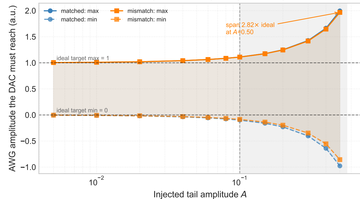
(d) Cost in AWG dynamic range: band height is the swing needed to place a unit-amplitude pulse on chip
