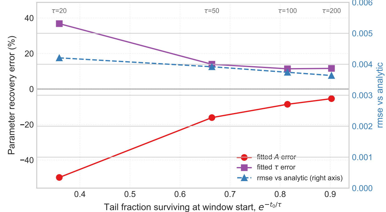
(d) Two orthogonal error sources: rmse is flat (artifact-dominated), recoverability tracks the surviving tail
