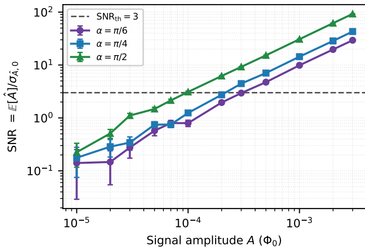
(c) SNR at N_{\text{shot}} = 10^4
