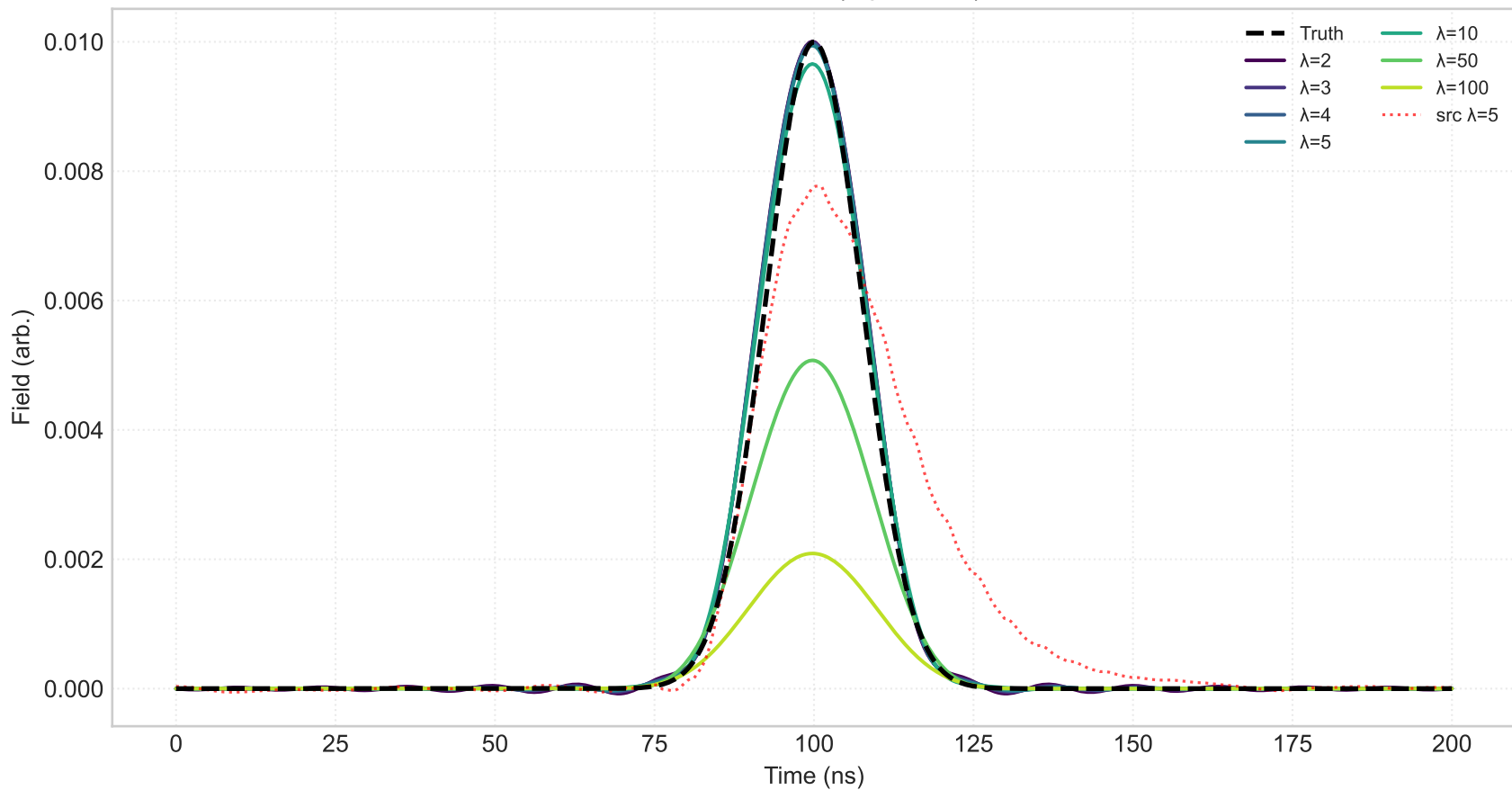
Wiener \lambda scan (sqc vs src)
