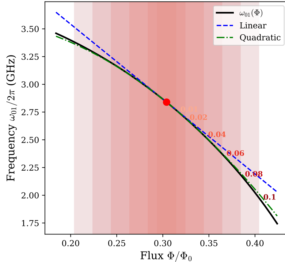
(b) Zoom at working point
