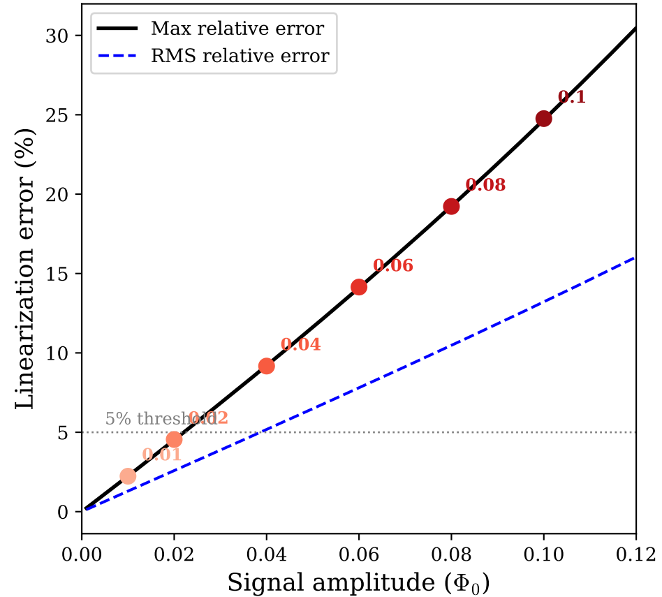
(c) Linear approx. error vs amplitude
