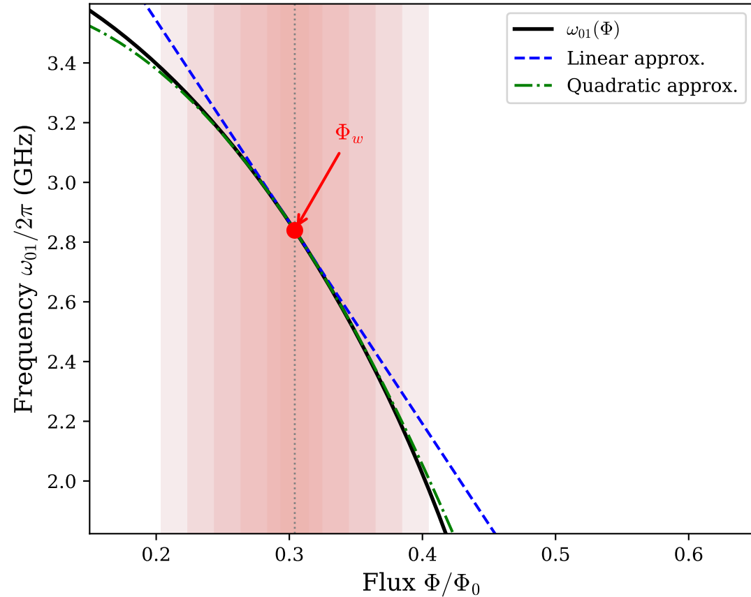
(a) Transmon frequency response
