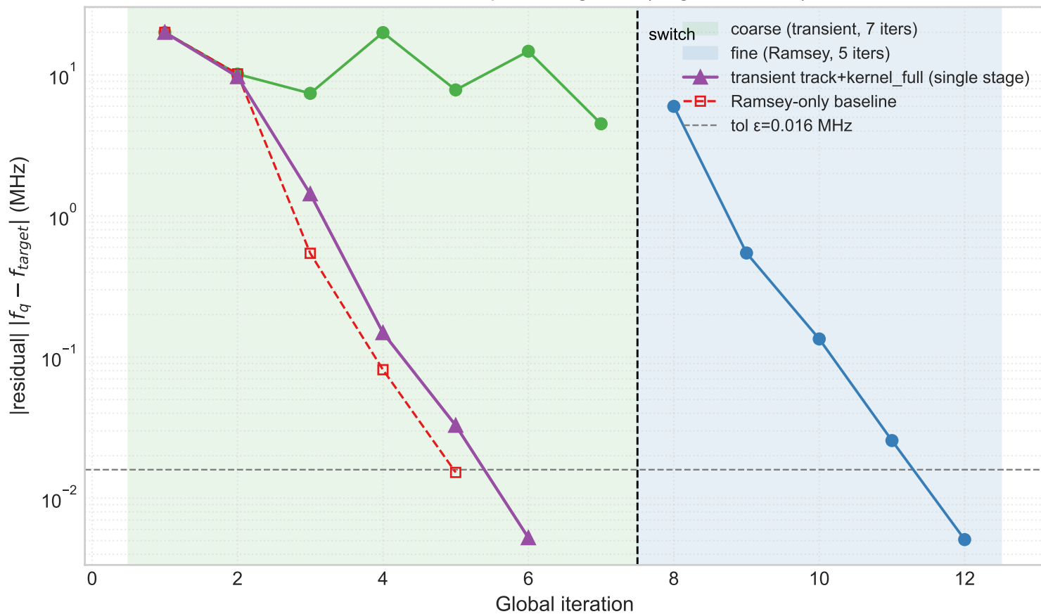
F4 — Closed-loop convergence (target -20 MHz)
