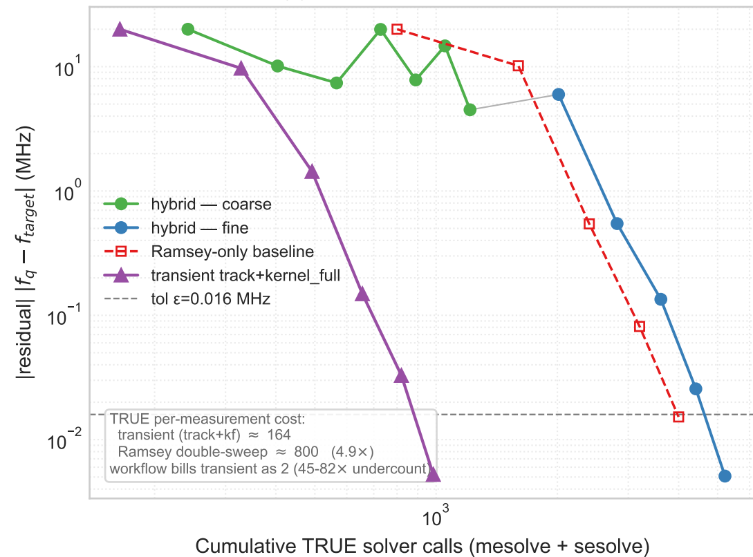
(a) Residual vs cumulative cost
