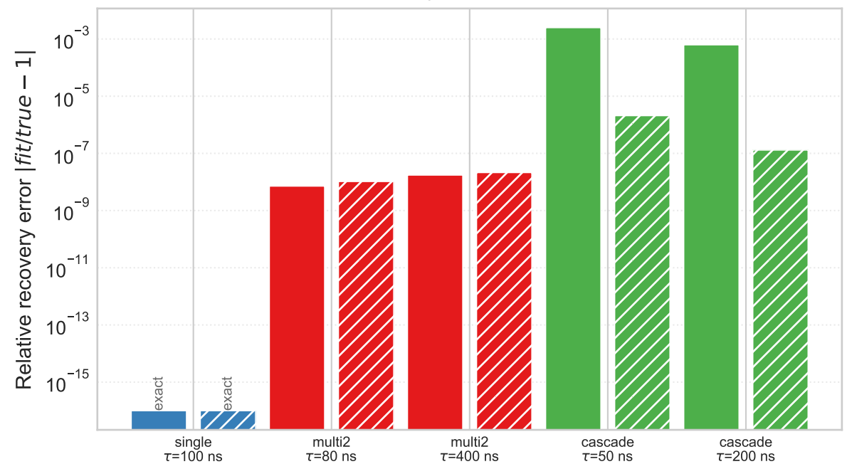
(d) Parameter recovery at K = K_{true} solid = amplitude, hatched = \tau
