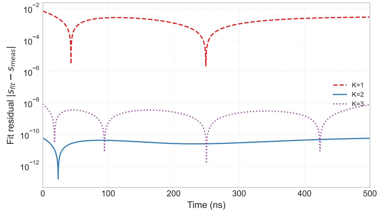
(b) Fit residual (log-y): the underfit floor is 8 orders above the correct order
