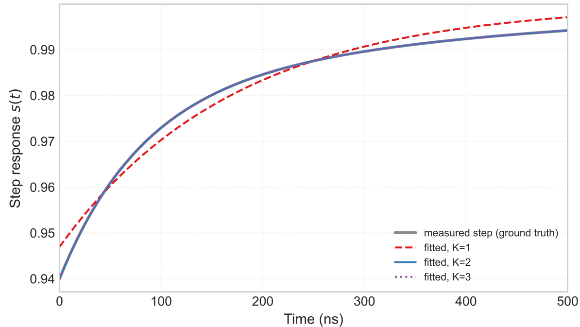
(a) Measured vs fitted step, 2-pole truth K=1 underfits; K=2 lands on the data
