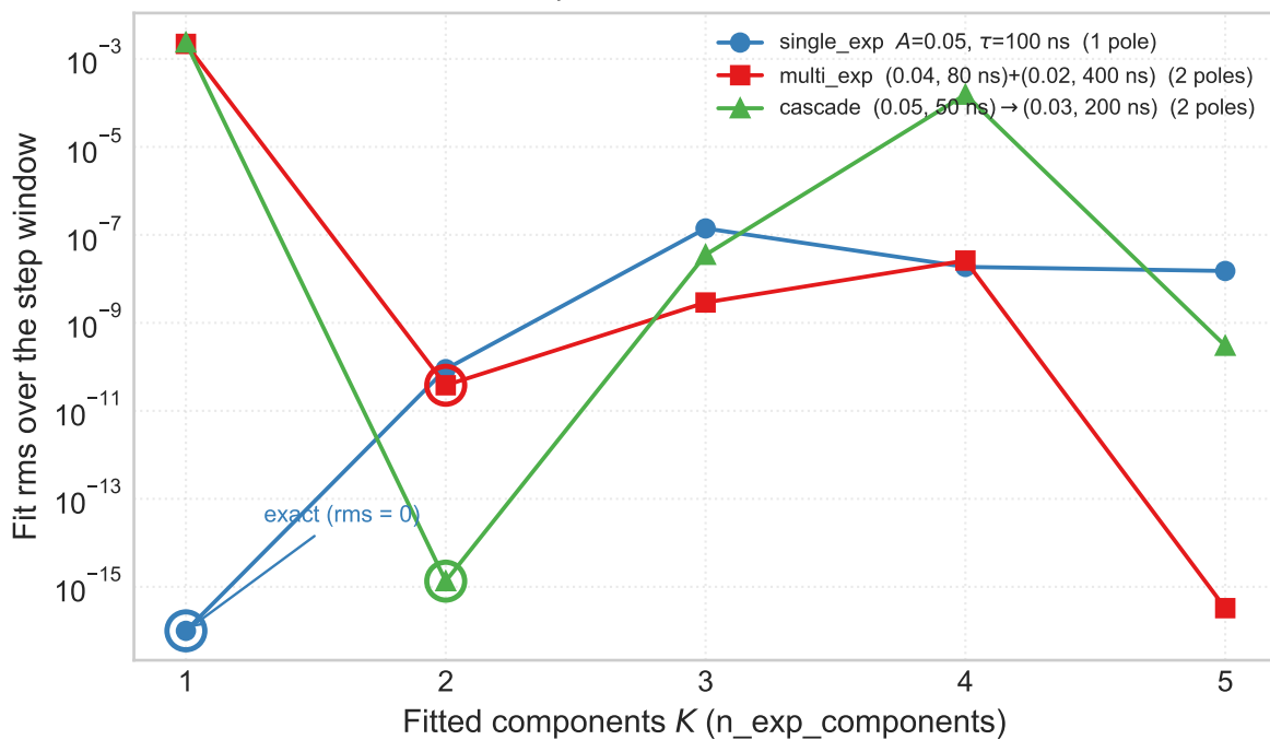
(c) Model-order selection (circled = true pole count) rms collapses at K = K_{true} , then scatters
