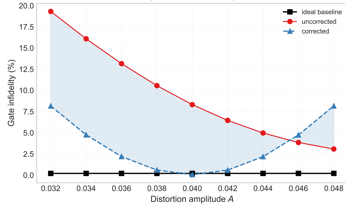
(d) Robustness to control-line drift (calibrated at A=0.040)
