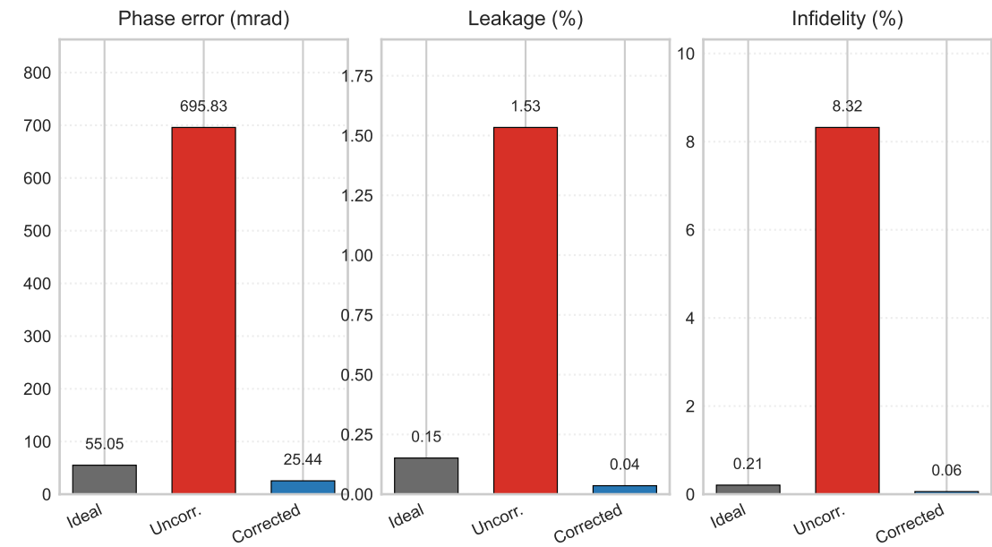
(d) Robustness to control-line drift (calibrated at A=0.040)
