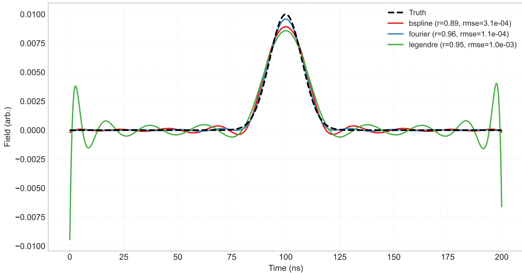
LM basis comparison (sqc, n_basis=20, \lambda=100 )
