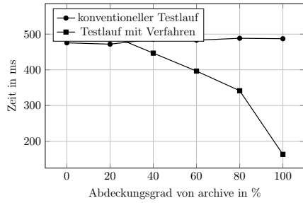
(c) wenige mittellange Testcases: T=10 , I=1000000
