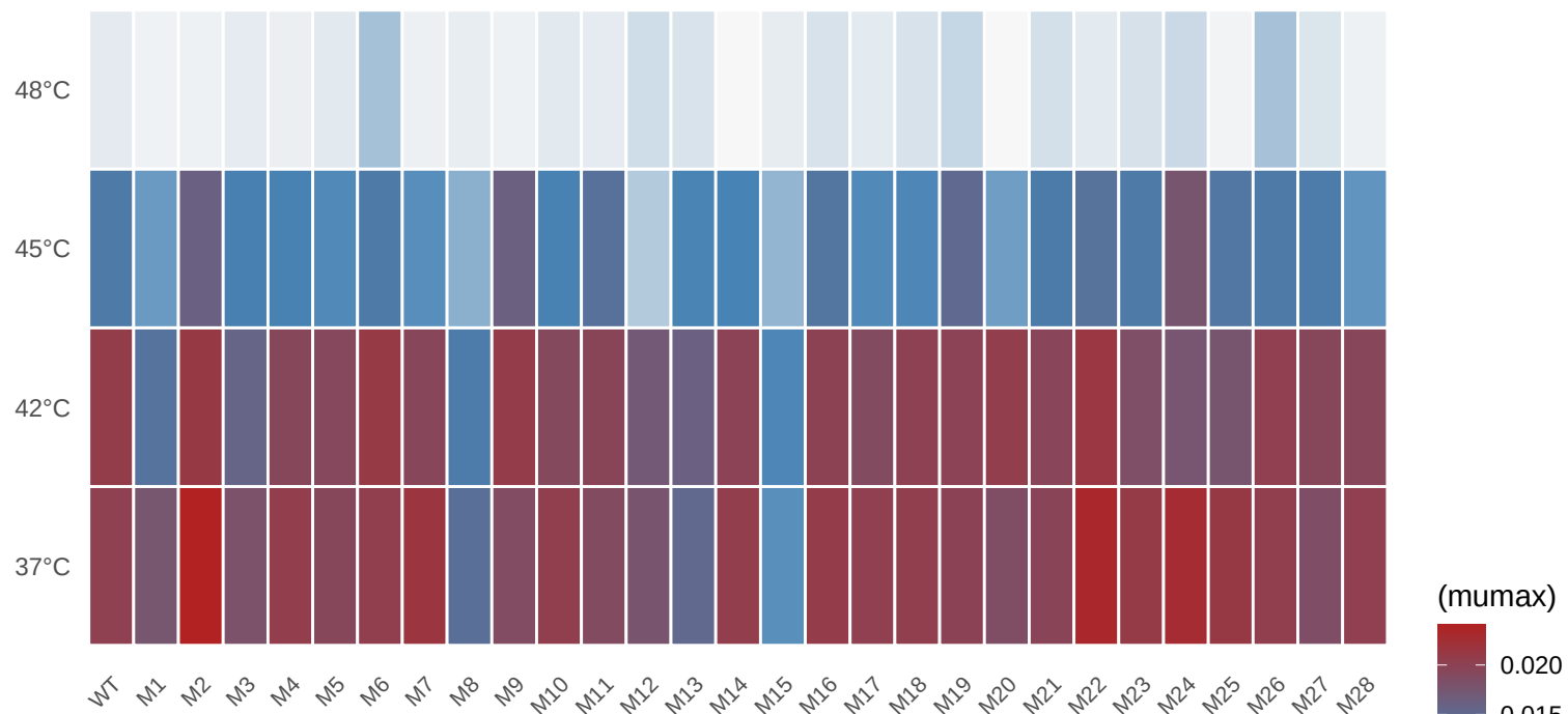
M9gluc
