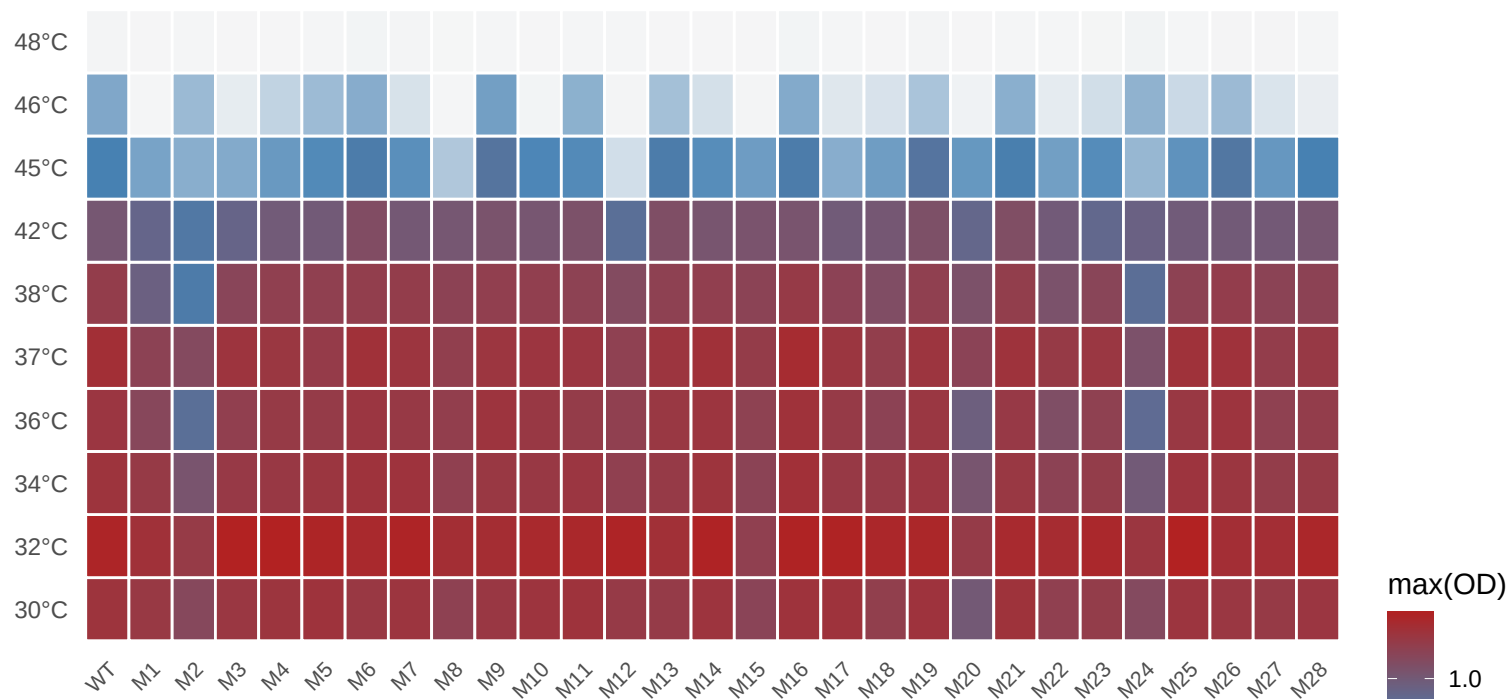
M9gluc
