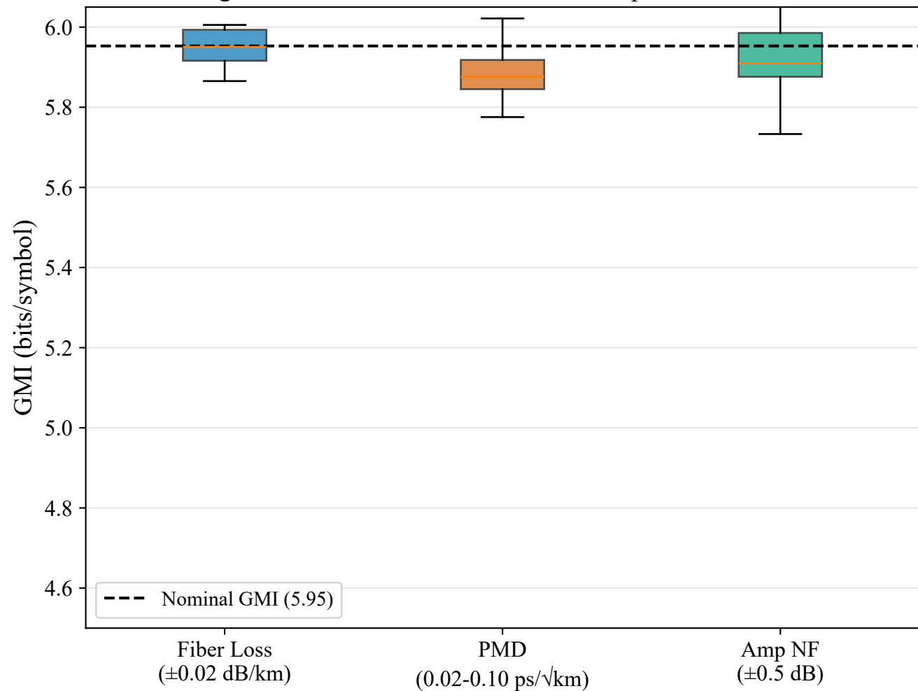
Fig 10. GMI Robustness to Fiber and Amplifier Variations
