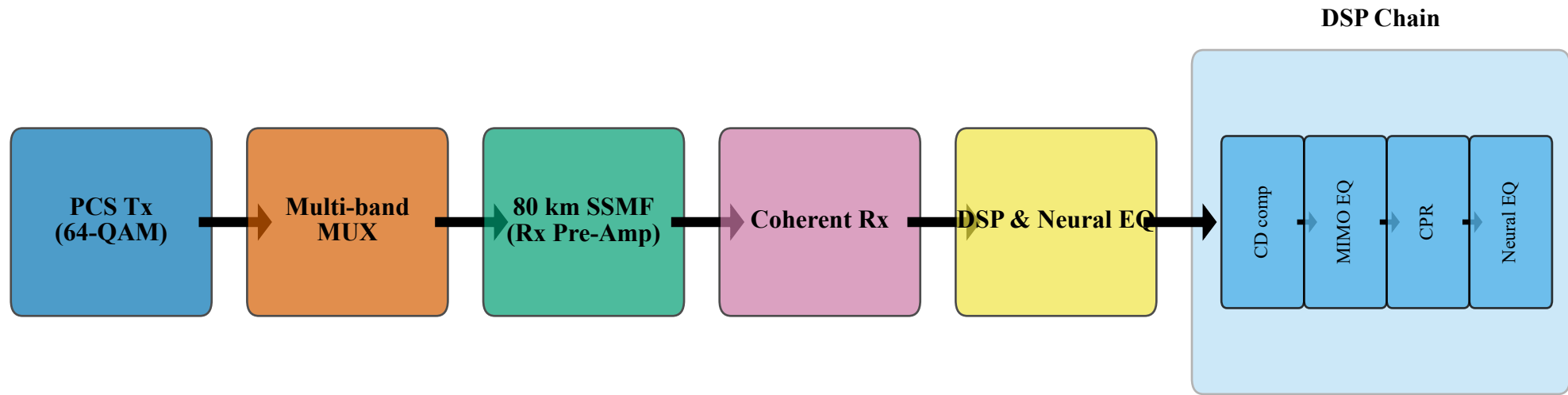
Fig 1. System Architecture for O+E+S+C+L Neural-PCS Transmission
