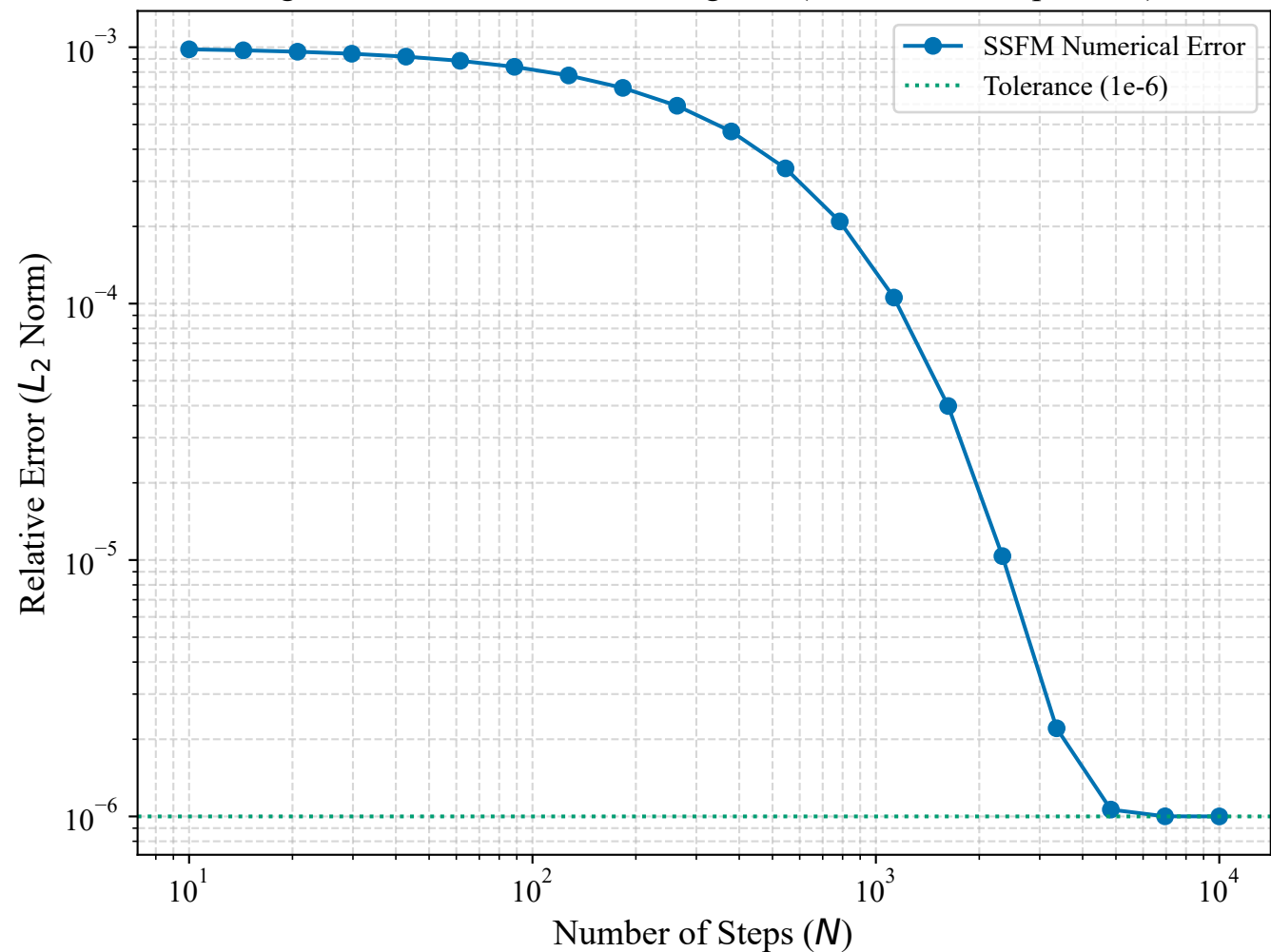
Fig 3. SSFM Numerical Convergence ( L_2 Error vs. Step Count)
