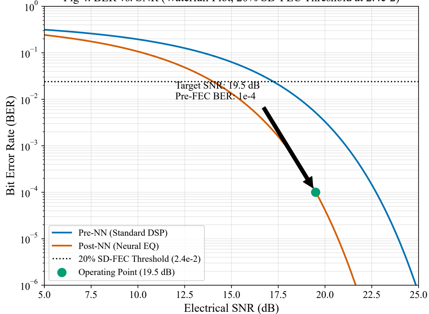
Fig 4. BER vs. SNR (Waterfall Plot, 20% SD-FEC Threshold at 2.4 \times 10^{-2} )
