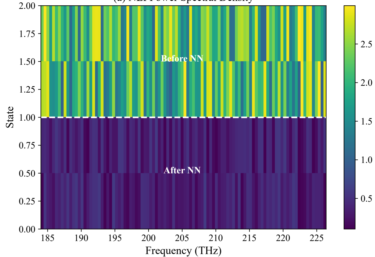
(a) NLI Power Spectral Density
