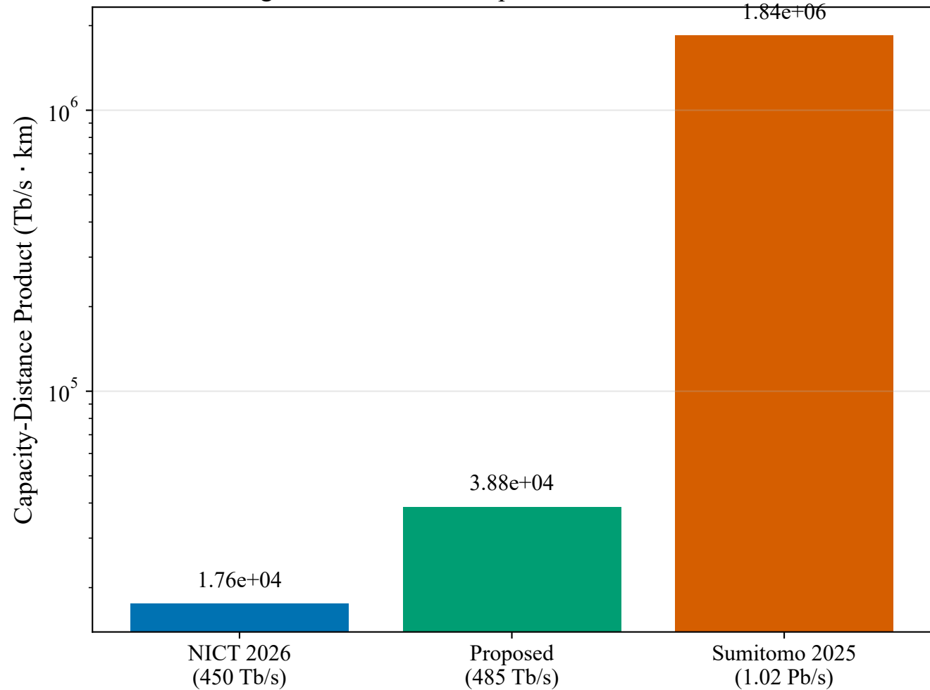
Fig 8. Performance Comparison vs. Recent Records
