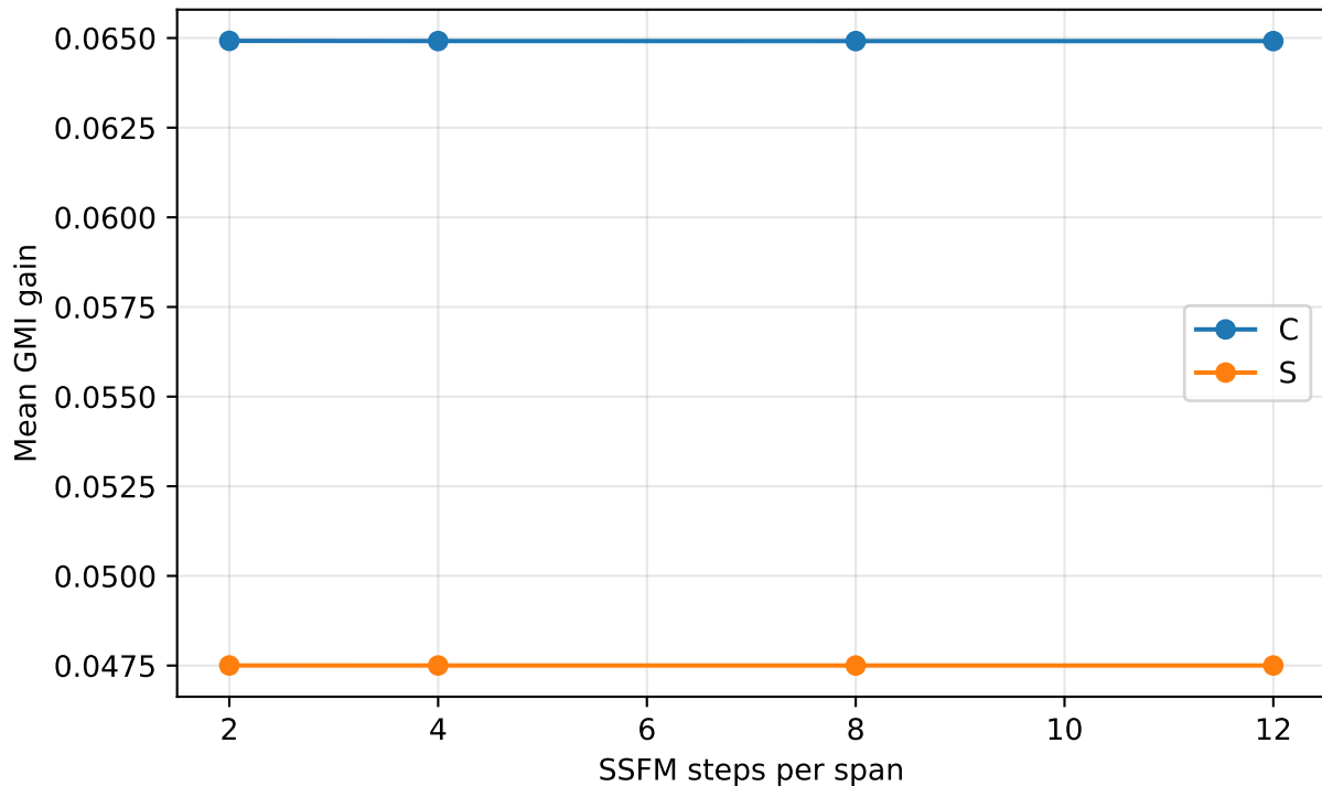
SSFM step-size convergence of PCS gain
