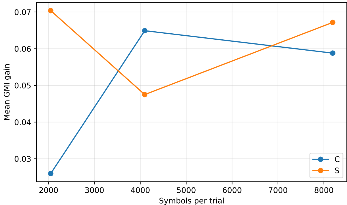
Symbol-count convergence of PCS gain
