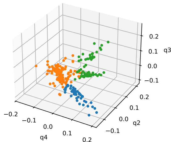
E-5: 3 strict nodal domains
