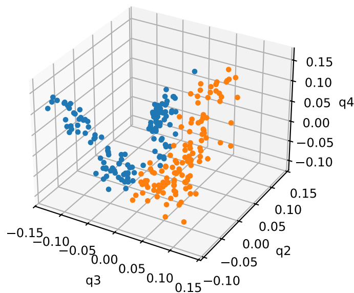
E-5: 2 strict nodal domains
