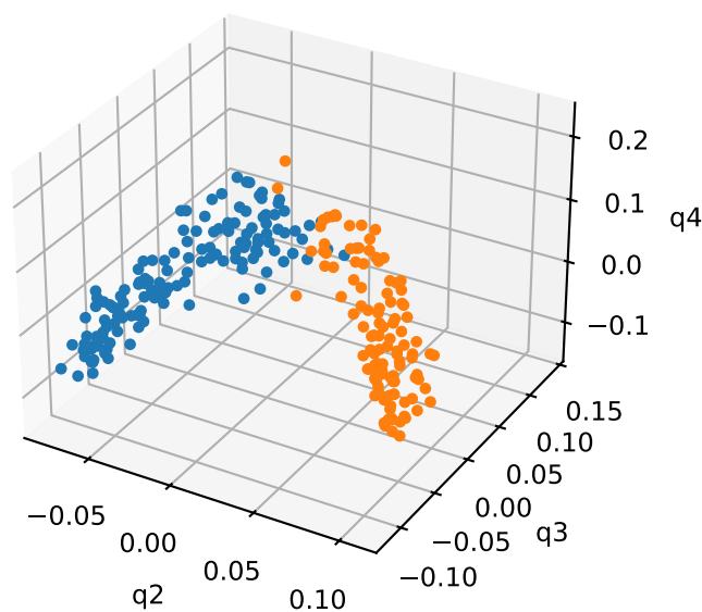
E-5: 2 strict nodal domains
