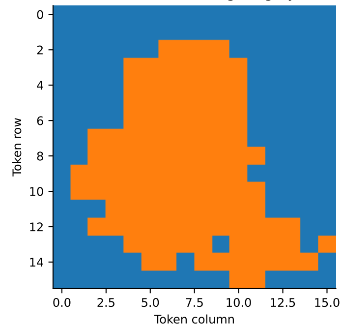
Nodal domains on token grid (gray: zero)
