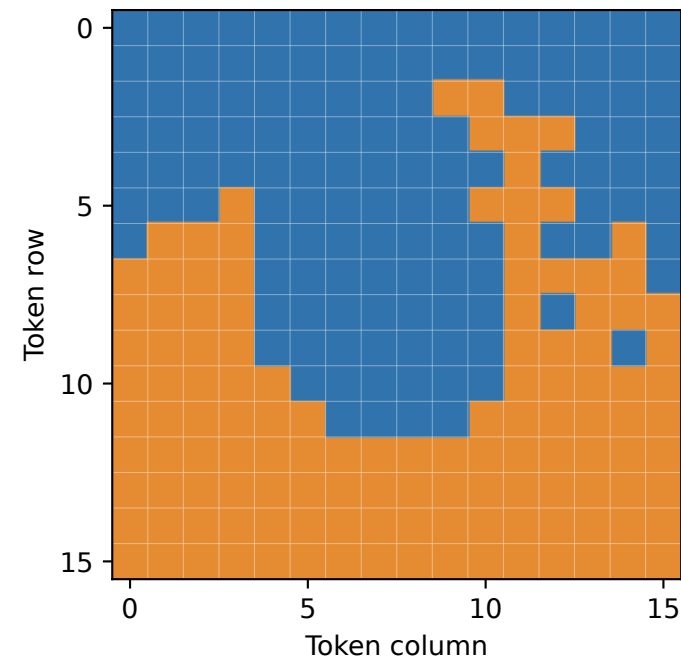
Selected nodal domains, q3 2 domains
