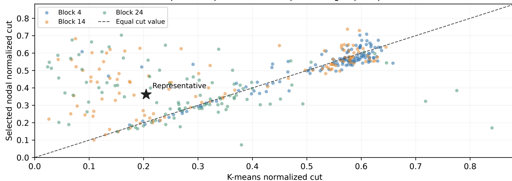
Descriptive comparison: 348 complete two-group snapshots
