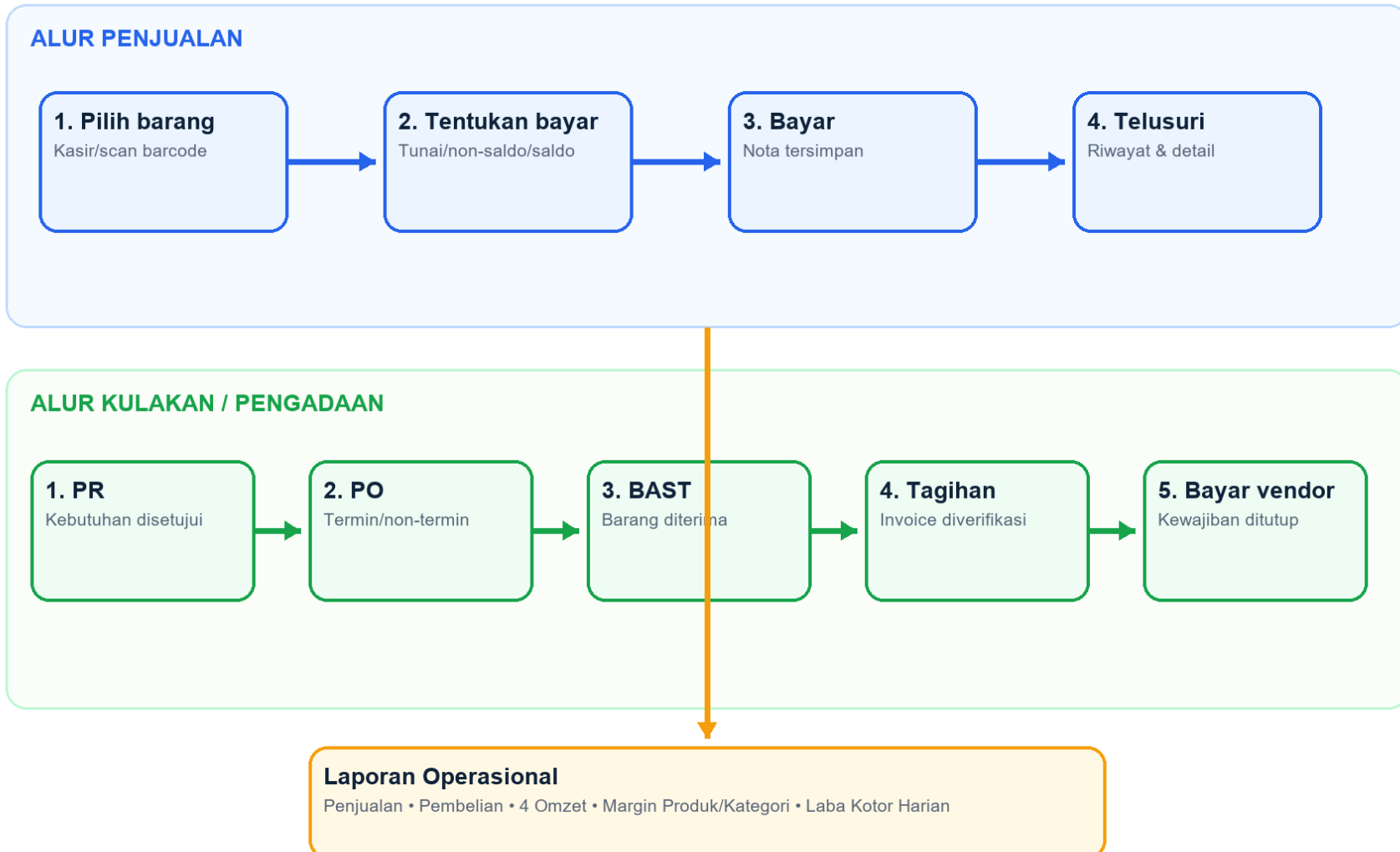
Diagram 1 — Alur End-to-End.
