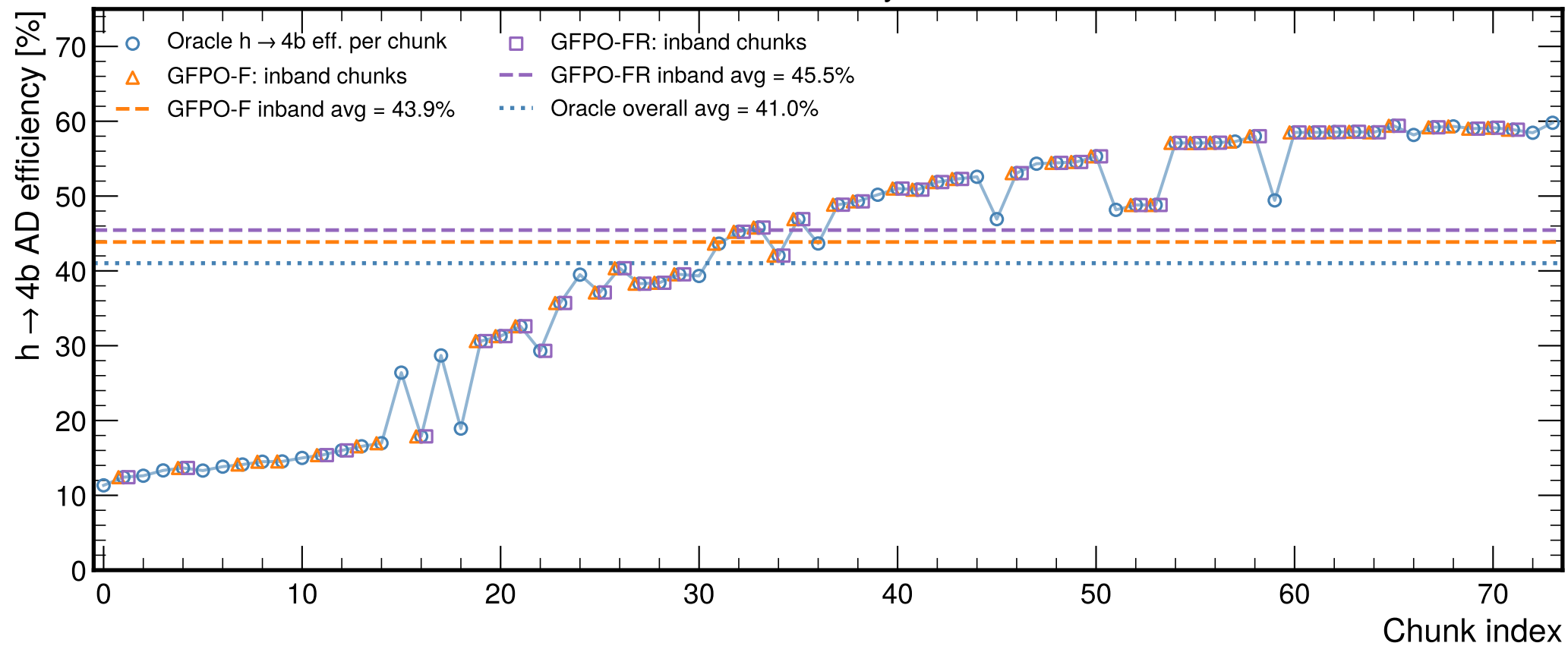
Per-chunk h \rightarrow 4b AD efficiency — CMS Run 283408
