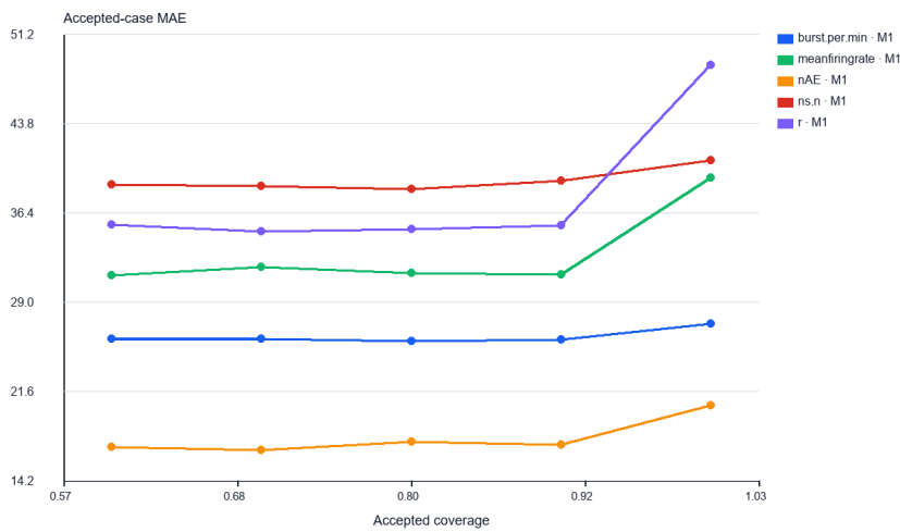
Risk-coverage: lower accepted-case MAE is better
