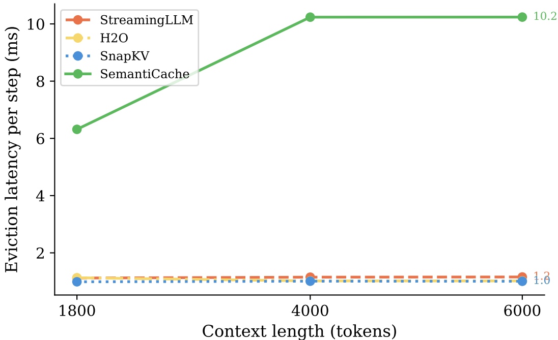
Eviction Overhead Scaling at b = 20\%
