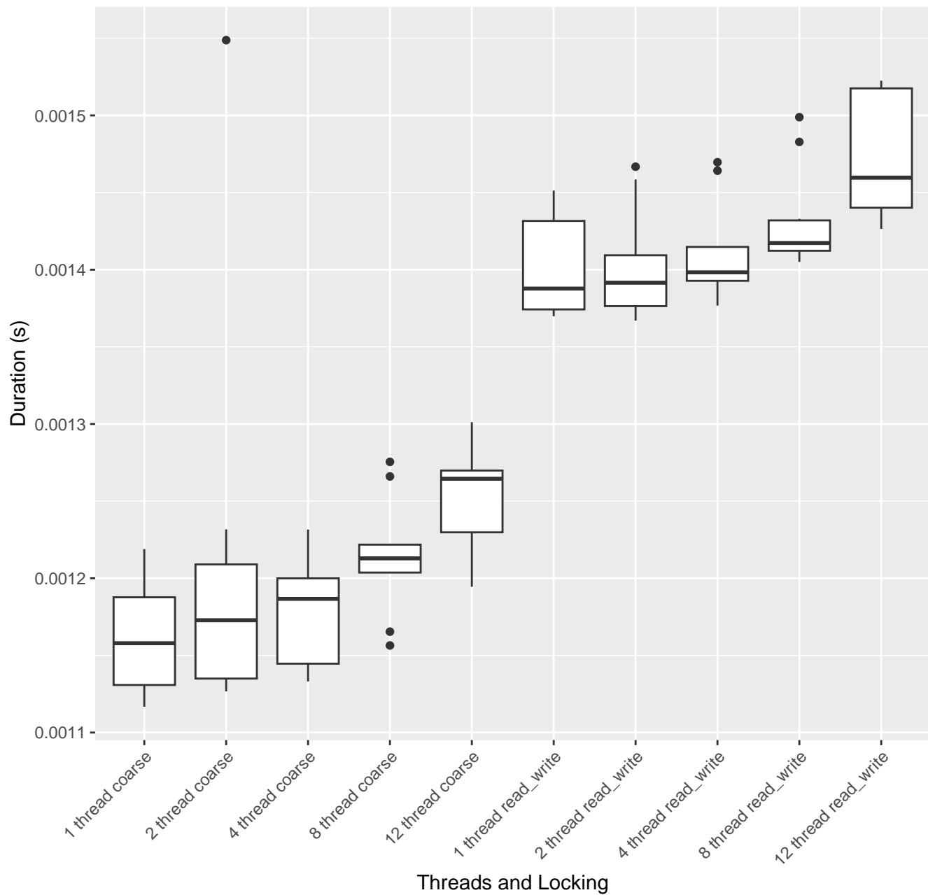
Read-only 1mil key performance by locking type and thread count
