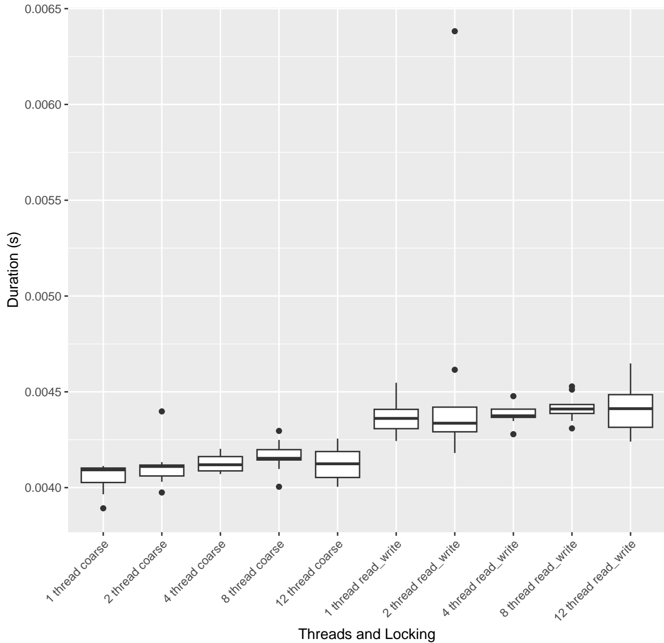
70/30 read/write 10k key performance by locking type and thread count
