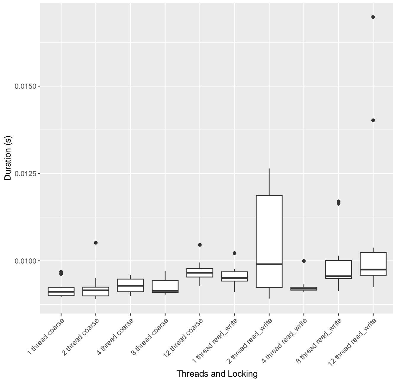
Write-only 10k key performance by locking type and thread count
