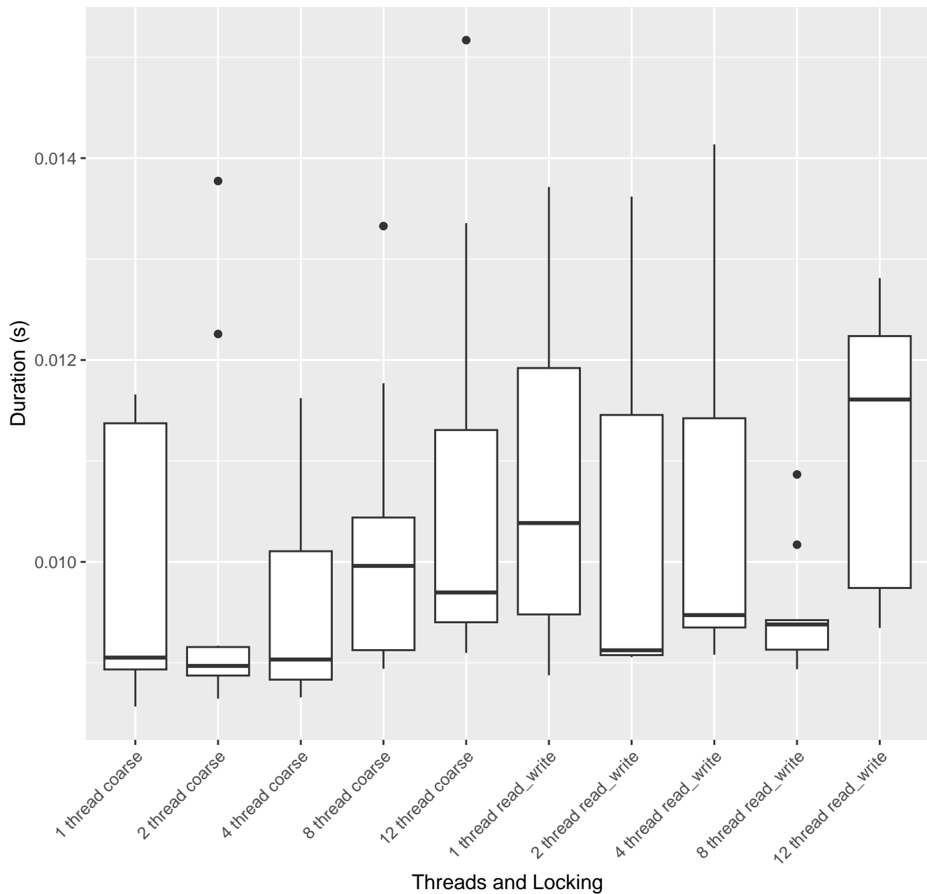
70/30 read/write 1mil key performance by locking type and thread count
