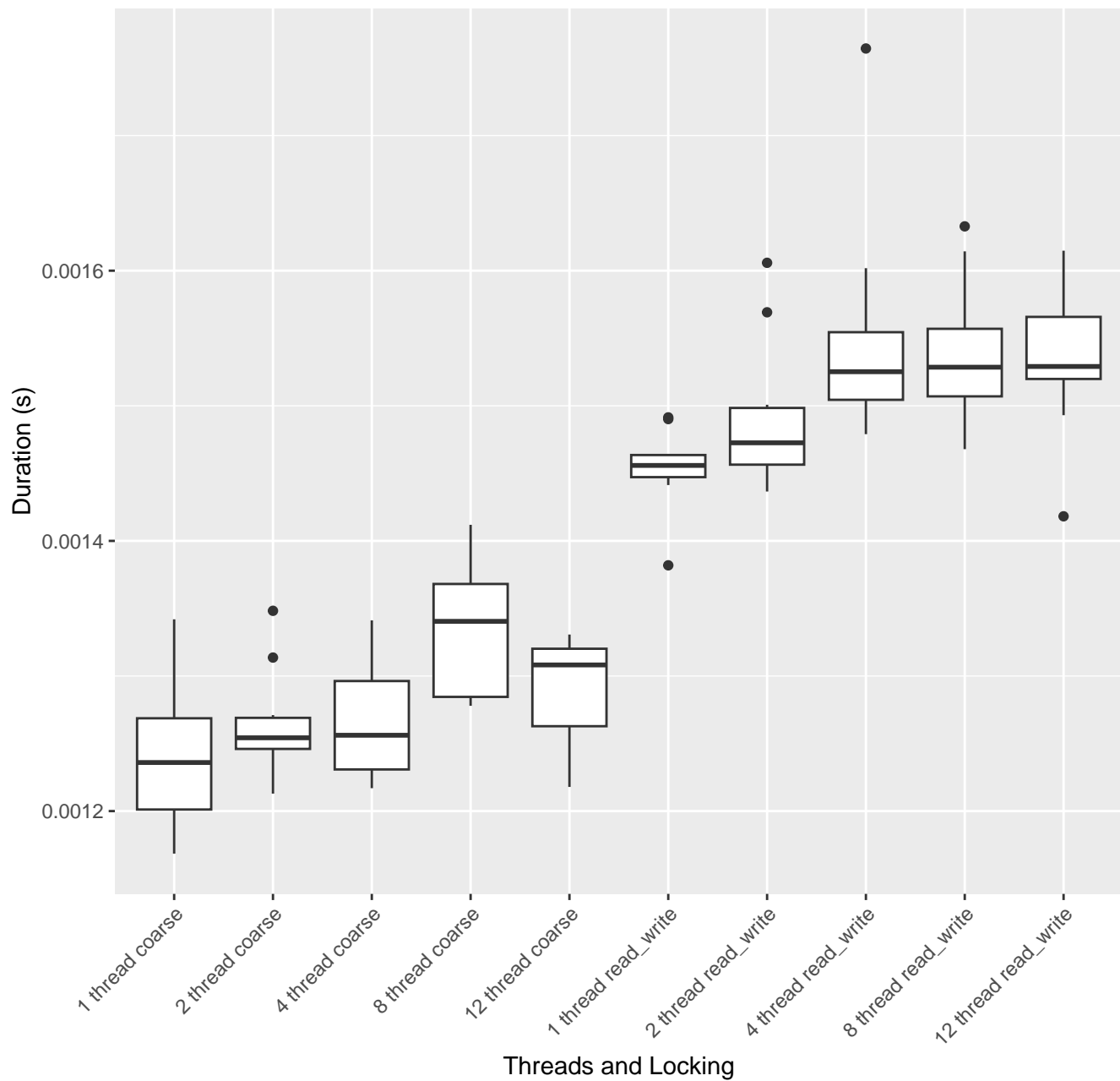
Read-only 10k key performance by locking type and thread count
