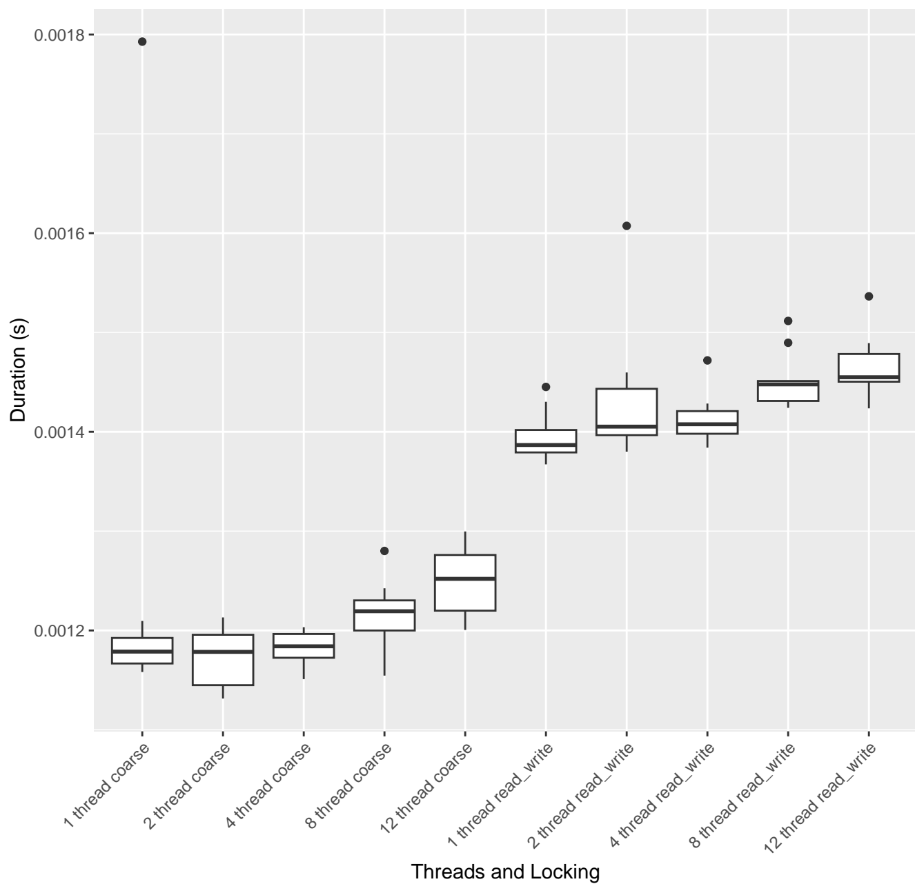
Read-only 100k key performance by locking type and thread count
