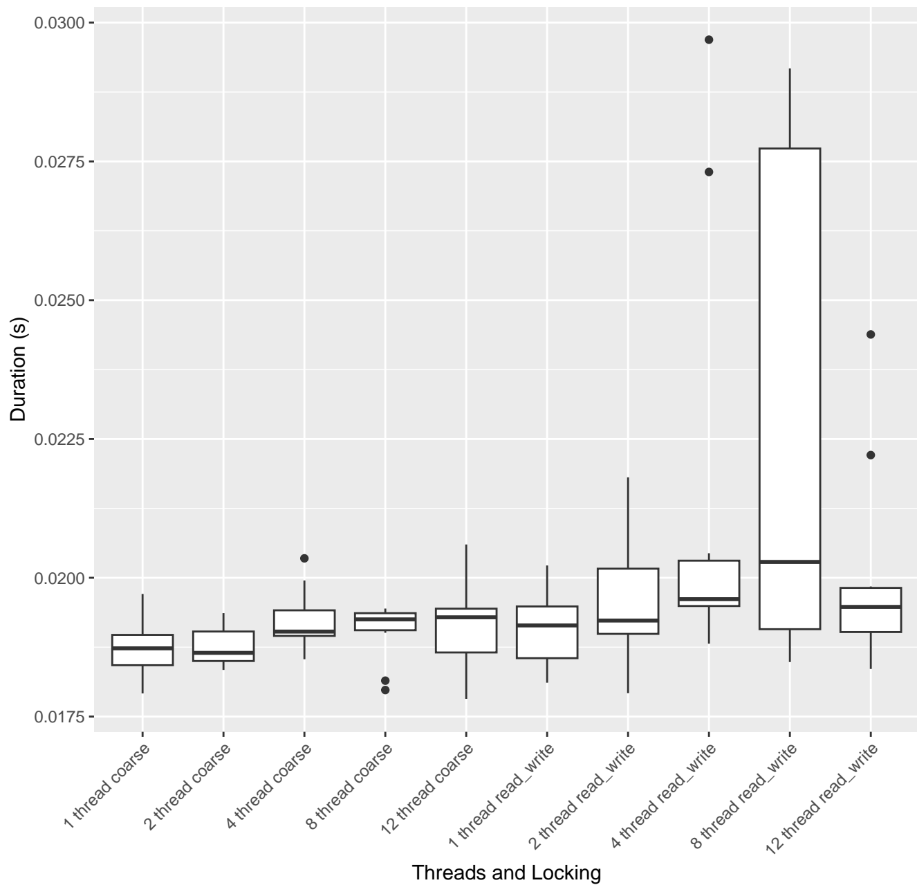
Write-only 100k key performance by locking type and thread count
