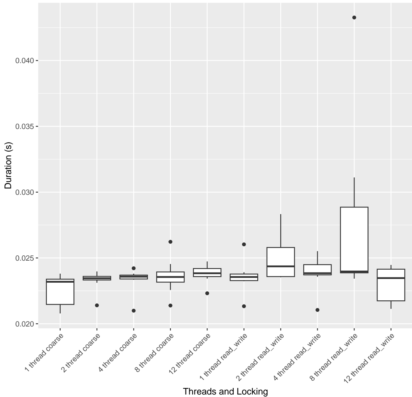
Write-only 1mil key performance by locking type and thread count
