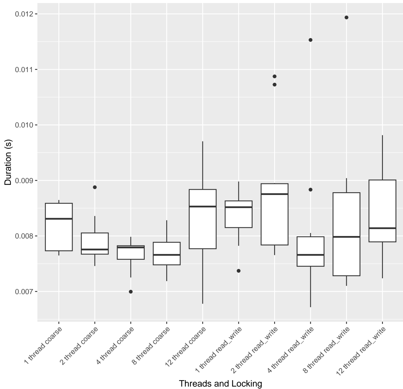
70/30 read/write 100k key performance by locking type and thread count
