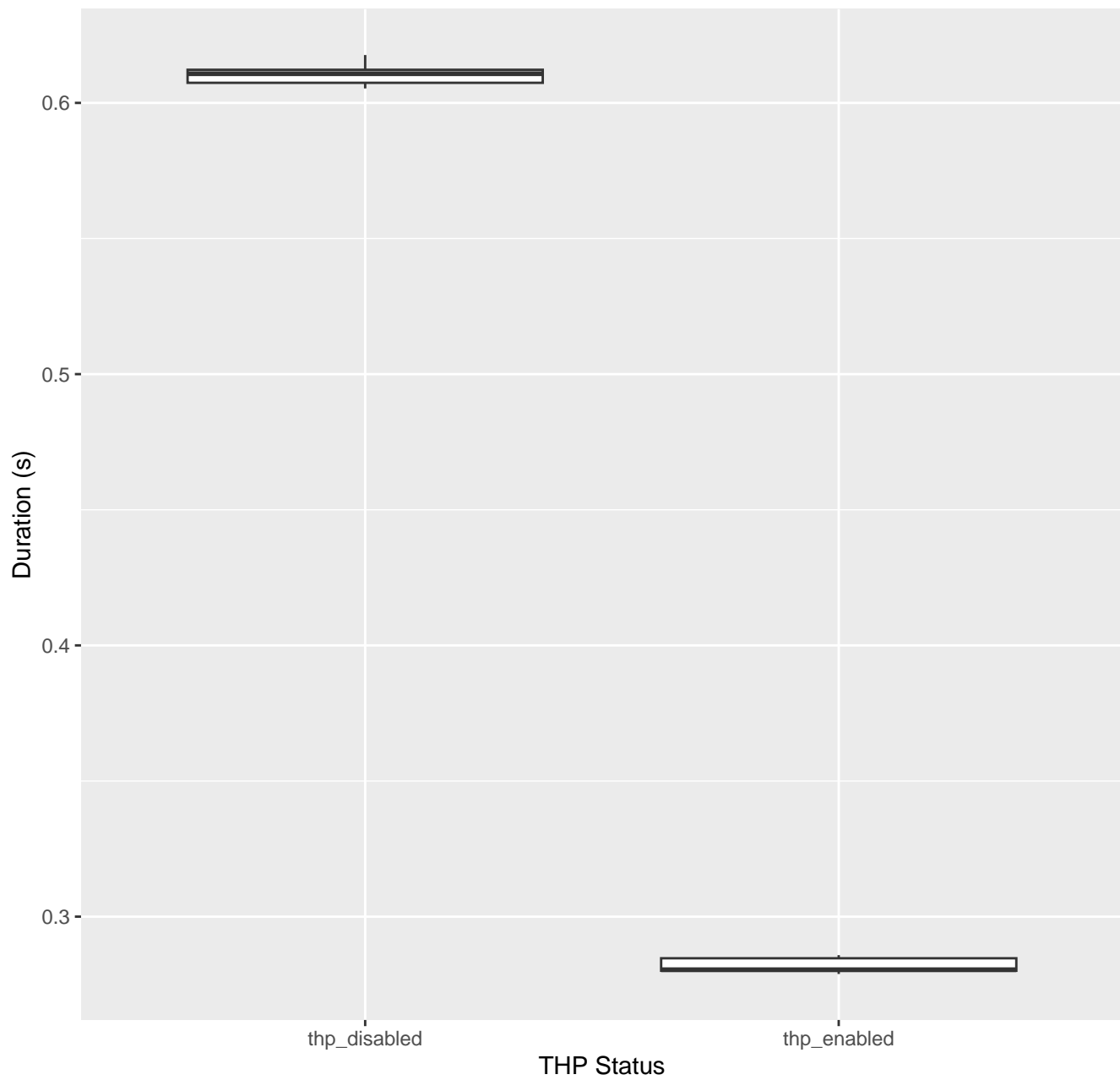
Memory Access Benchmark with and without THP
